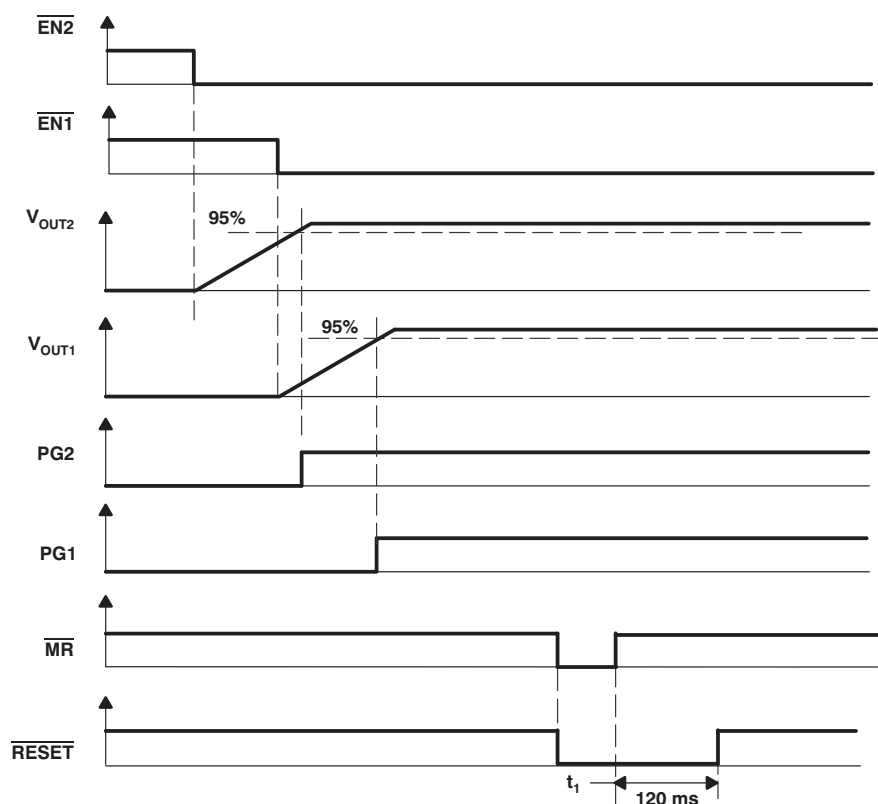
Figure 39. Timing When \overline{\text{MR}} is Toggled
