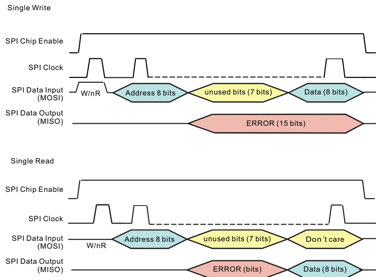
Figure 7-18. SPI READ and WRITE Protocol
