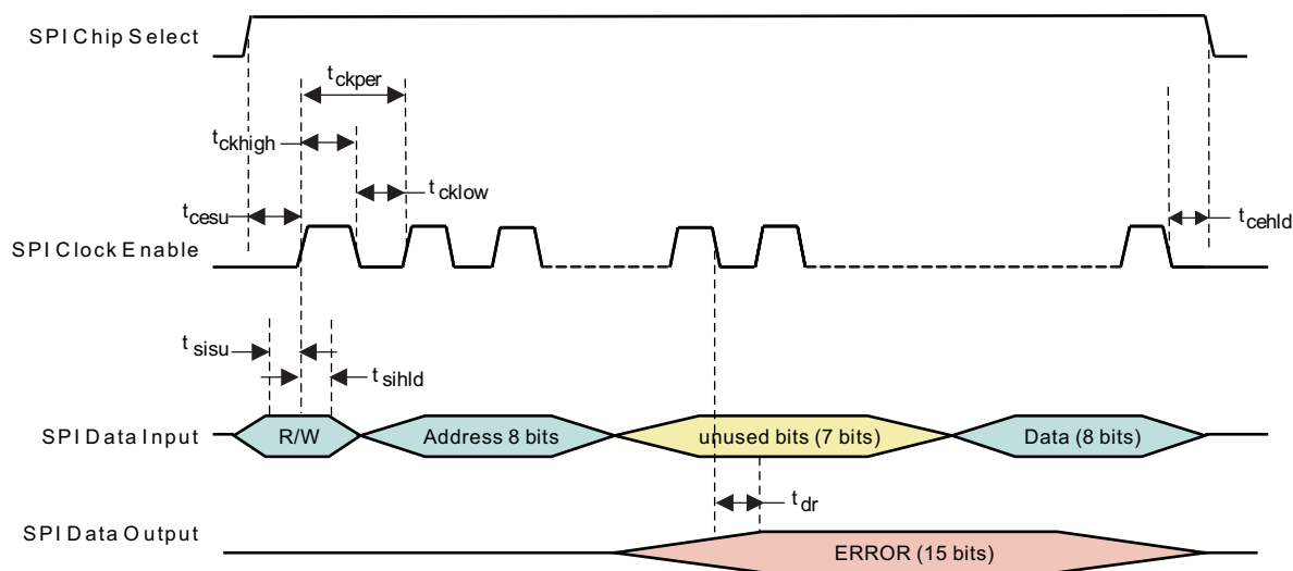
Figure 6-3. SPI Interface Timing
