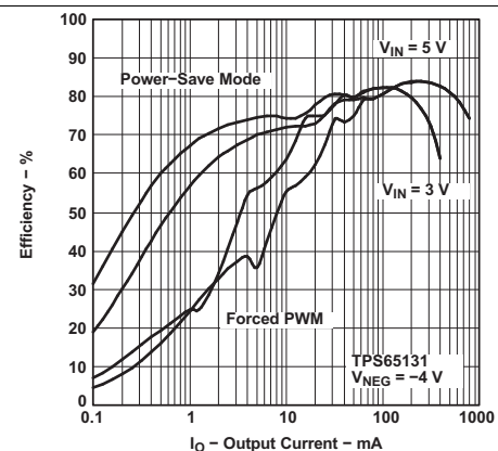
Figure 16. TPS65131 Efficiency vs Output Current
