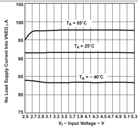
Figure 7. No Load Supply Current into V_{\text{NEG}} vs Input Voltage
