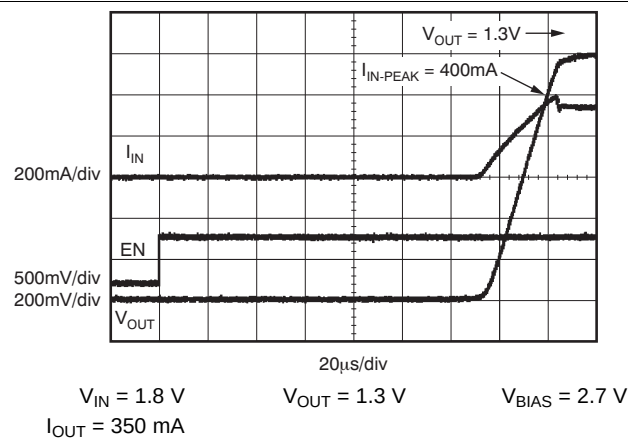
Figure 23. VIN Inrush Current
