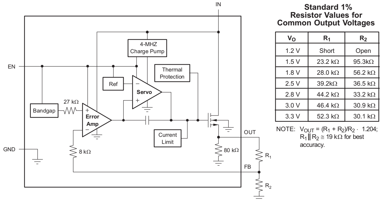
Figure 30. Adjustable-Voltage Version
