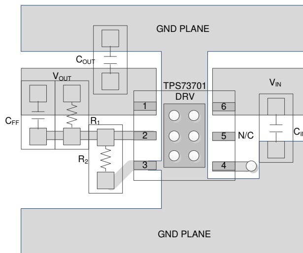
Figure 39. Layout Example
