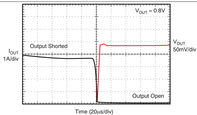
Figure 25. Output Short-Circuit Recovery
