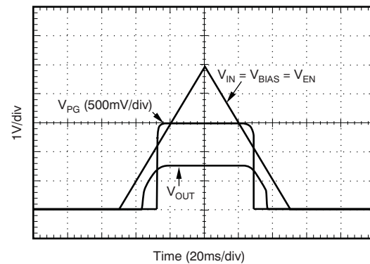
Figure 29. Power-Up, Power-Down
