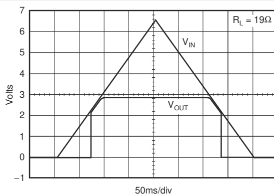
Figure 6-25. TPS799285 Power-Up and Power-Down
