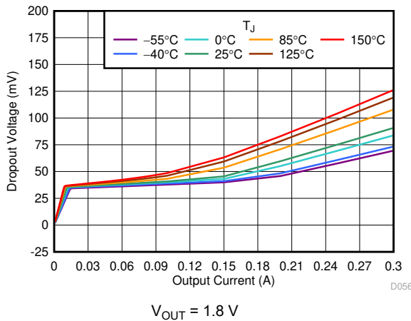
图 6-5. Dropout Voltage vs I_{OUT}
