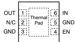
DRV PACKAGE 2-mm x 2-mm SON-6 (TOP VIEW)
