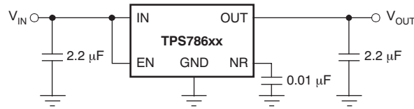
Figure 27. Typical Application Circuit
