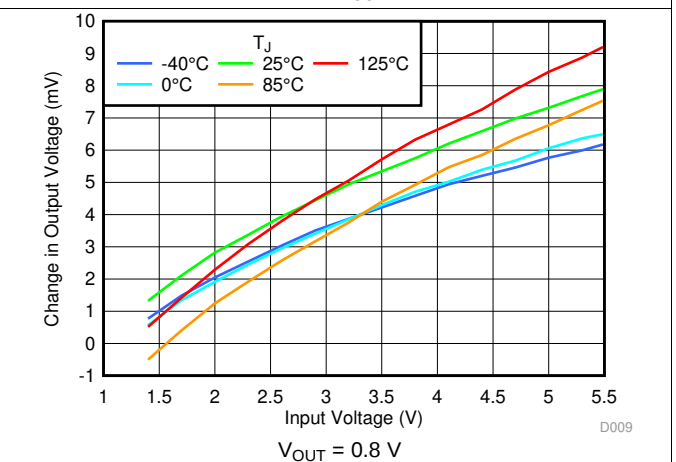
图 24. Line Regulation V_{IN} and Temperature
