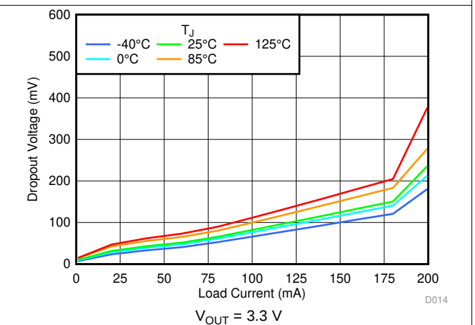
图 22. Dropout vs I_{OUT} and Temperature
