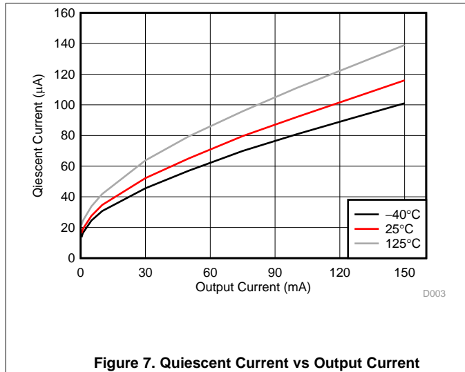
Figure 7. Quiescent Current vs Output Current
