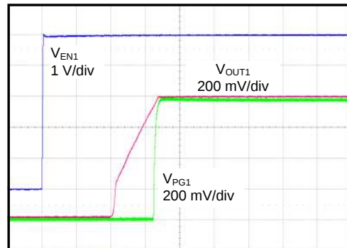
图 20. Start-Up ( \text{SS\_CTRLX} = \text{GND} , C_{\text{NR/SSX}} = 0\text{ nF} )
