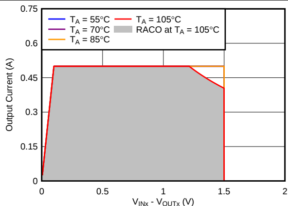
图 61. Recommended Area for Continuous Operation for V_{OUTx} = 5.0\text{ V}
