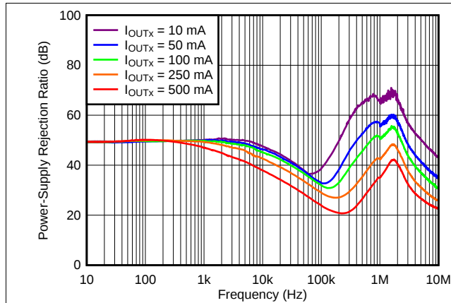
图 63. Power-Supply Rejection Ratio vs Frequency
