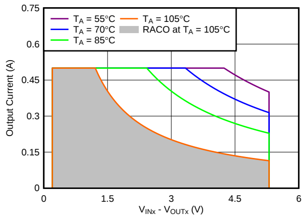
图 57. Recommended Area for Continuous Operation for V_{OUTx} = 1.2\text{ V}
