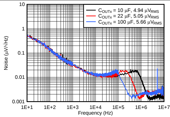
图 13. Noise vs Frequency and C_{\text{OUTX}}
