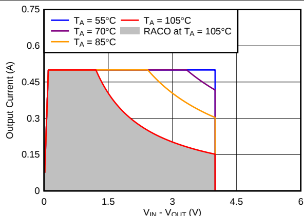
图 59. Recommended Area for Continuous Operation for V_{OUTx} = 2.5\text{ V}
