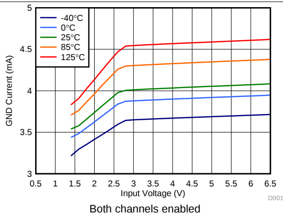
图 33. Ground Current vs Input Voltage
