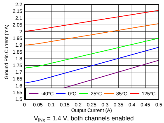
图 32. Ground Current vs Output Current
