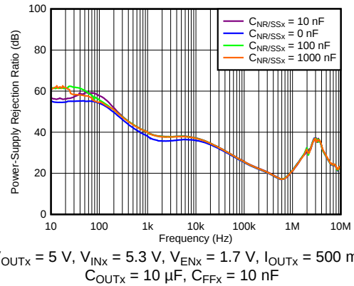
图 2. Power-Supply Rejection Ratio vs Frequency and C_{\text{NR/SSX}}
