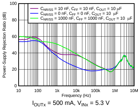
图 1. Power-Supply Rejection Ratio at V_{\text{OUTX}} = 5.0\text{ V}
