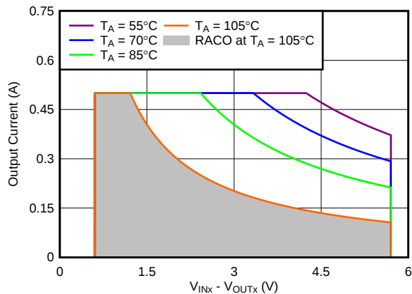
图 56. Recommended Area for Continuous Operation for V_{OUTx} = 0.8\text{ V}
