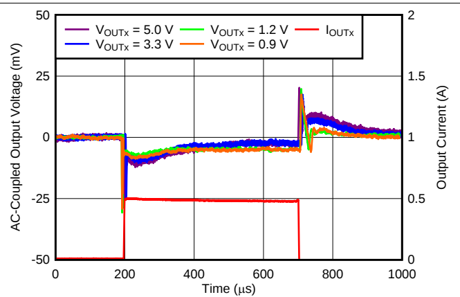
图 64. Load Transient Response vs Time and V_{OUTx}
