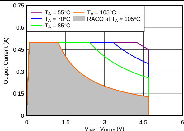
图 58. Recommended Area for Continuous Operation for V_{OUTx} = 1.8\text{ V}
