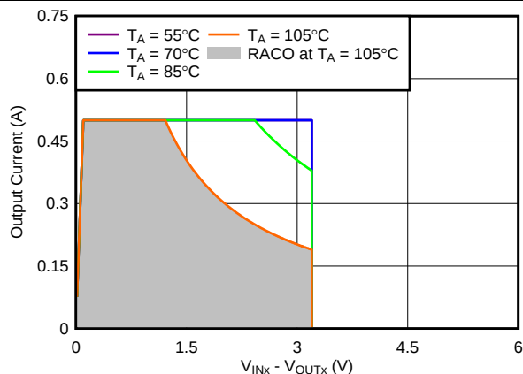
图 60. Recommended Area for Continuous Operation for V_{OUTx} = 3.3\text{ V}
