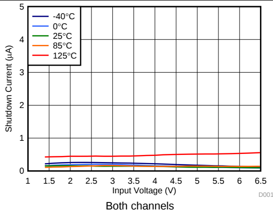
图 31. Shutdown Current vs Input Voltage
