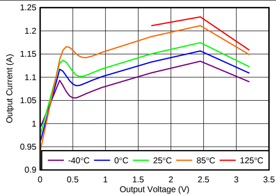
图 19. Current Limit Foldback
