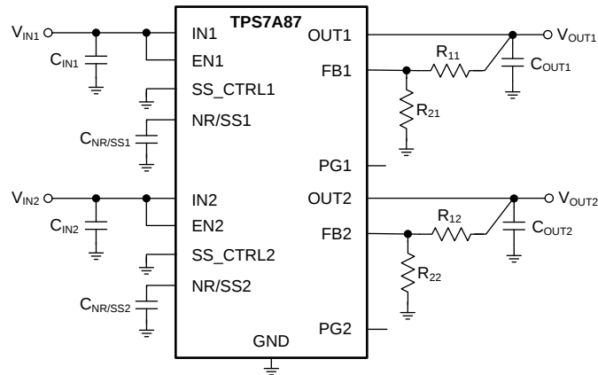
图 45. Adjustable Operation
