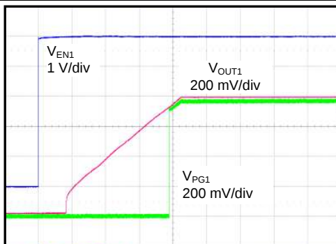
图 21. Start-Up ( \text{SS\_CTRLX} = \text{GND} , C_{\text{NR/SSX}} = 10\text{ nF} )
