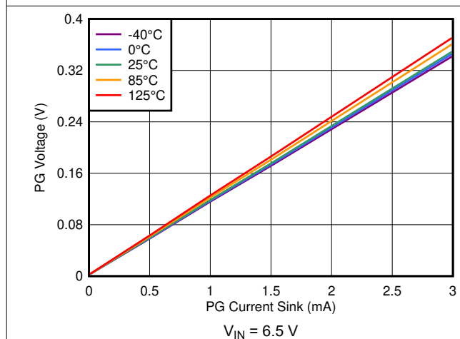
图 7-41. PG Voltage vs PG Current Sink
