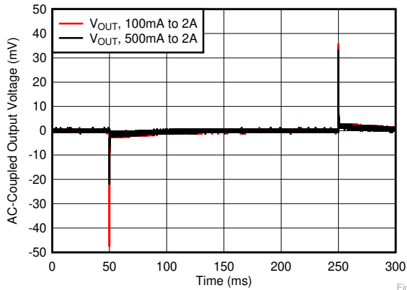
Fig1 V_{IN} = 5.3\text{ V} , V_{BIAS} = 5\text{ V} , C_{OUT} = 22\ \mu\text{F} , C_{BIAS} = 10\ \mu\text{F} , V_{OUT} = 5\text{ V} , C_{NR/SS} = C_{FF} = 10\text{ nF} , slew rate = 1\text{ A}/\mu\text{s}
