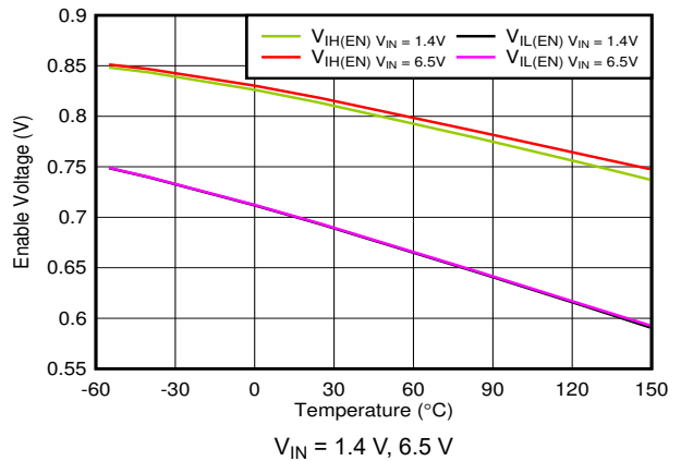
图 7-64. Enable Threshold vs Temperature
