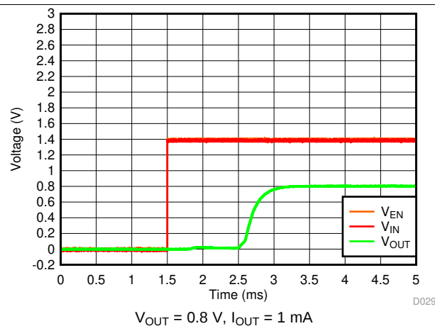
图 30. Startup With V_{EN} = V_{IN}
