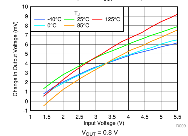
图 24. Line Regulation V_{IN} and Temperature
