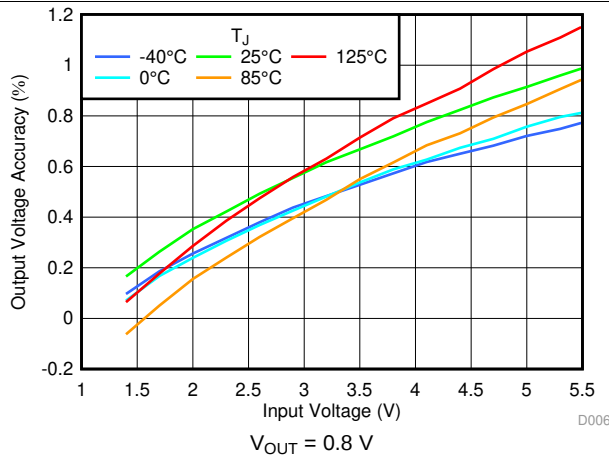
图 25. Output Accuracy V_{IN} and Temperature
