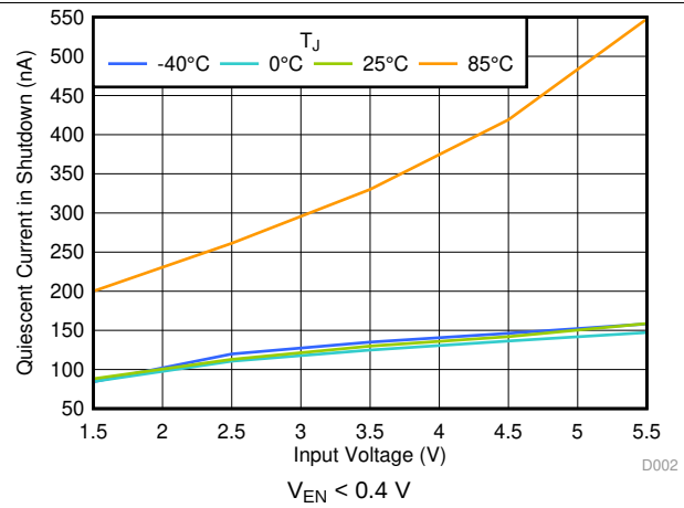
图 2. I_{SHDN} vs V_{IN} and Temperature
