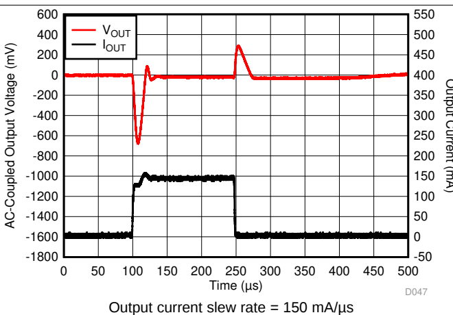
图 10. I_{OUT} Transient 0 mA to 150 mA
