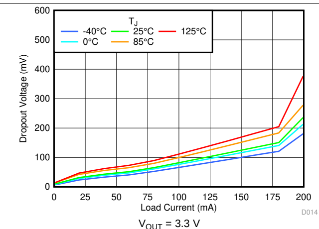
图 22. Dropout vs I_{OUT} and Temperature
