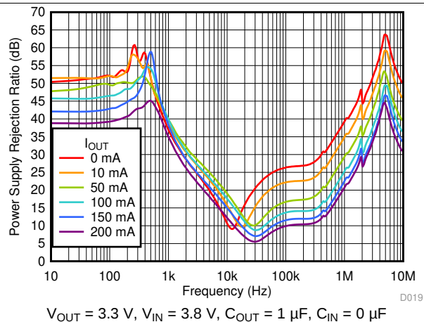
图 41. PSRR vs Frequency and I_{OUT}
