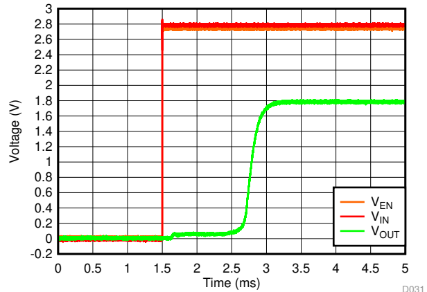
图 32. Startup With V_{EN} = V_{IN}
