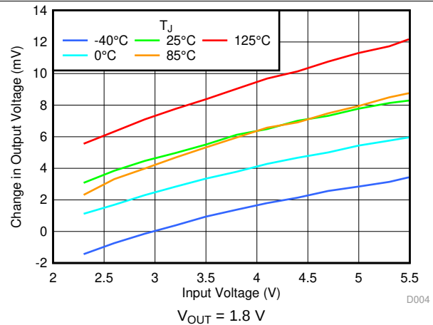
图 26. Line Regulation V_{IN} and Temperature
