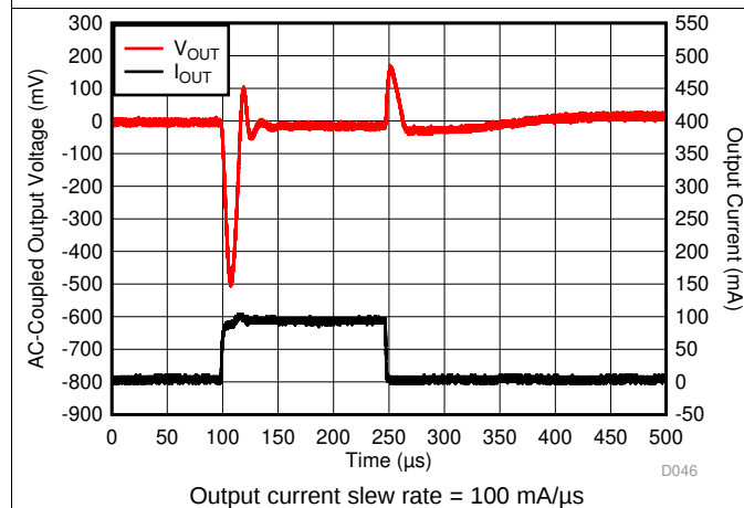
图 9. I_{OUT} Transient 0 mA to 100 mA
