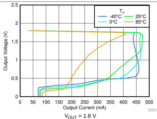
图 29. Foldback Current Limit vs I_{OUT} and Temperature
