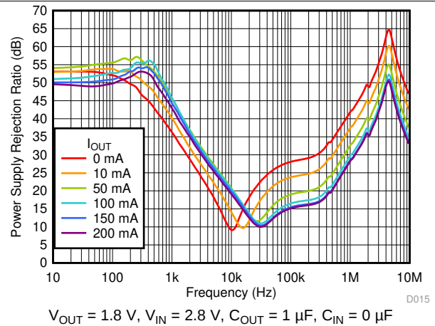
图 40. PSRR vs Frequency and I_{OUT}
