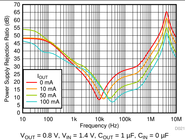
图 39. PSRR vs Frequency and I_{OUT}
