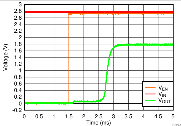
图 33. Startup With Separate V_{IN} and V_{EN}
