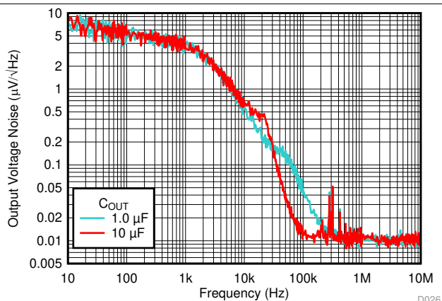
图 44. Output Noise vs Frequency and C_{OUT}
