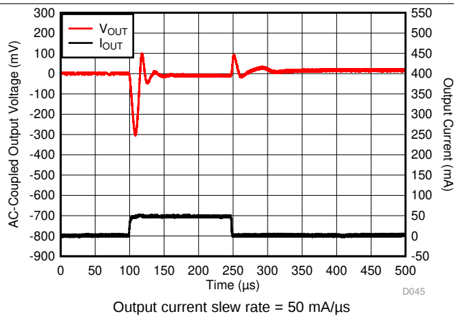
图 8. I_{OUT} Transient 0 mA to 50 mA
