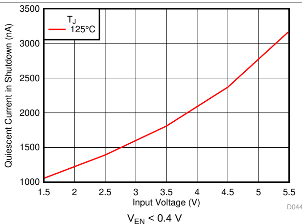
图 3. I_{SHDN} vs V_{IN} and Temperature
