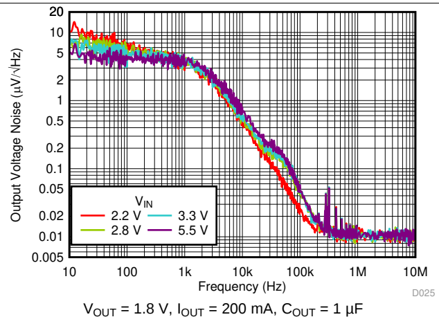
图 42. Output Noise vs Frequency and V_{IN}
