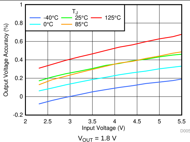
图 27. Output Accuracy V_{IN} and Temperature
