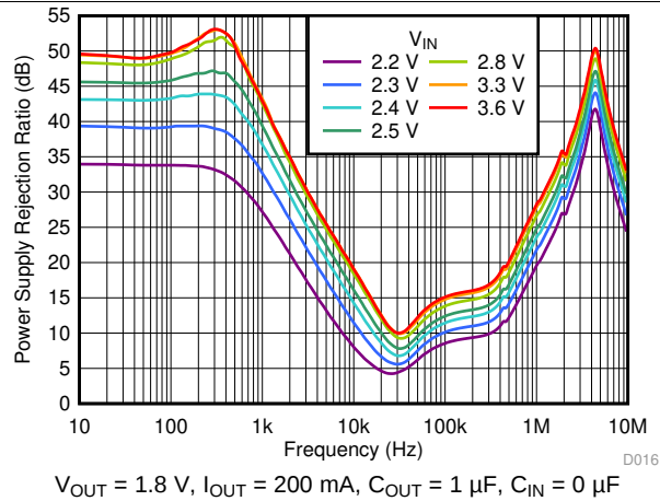
图 37. PSRR vs Frequency and V_{IN}
