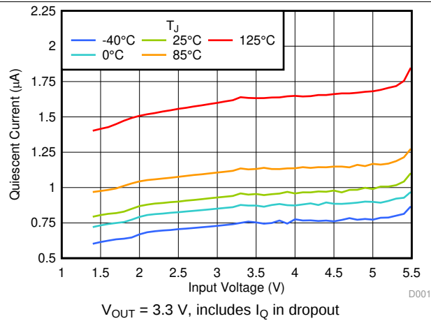
图 1. I_Q vs V_{IN} and Temperature
