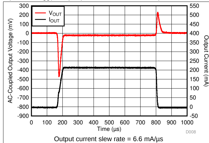
图 7. I_{OUT} Transient 0 mA to 200 mA
