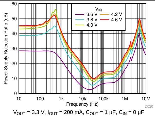
图 38. PSRR vs Frequency and V_{IN}
