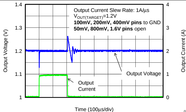
Figure 30. Load Transient Response (V OUT = 1.2 V)
