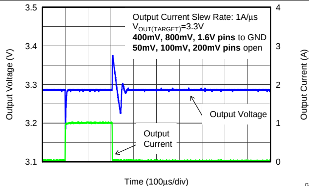
Figure 31. Load Transient Response (V OUT = 3.3 V)
