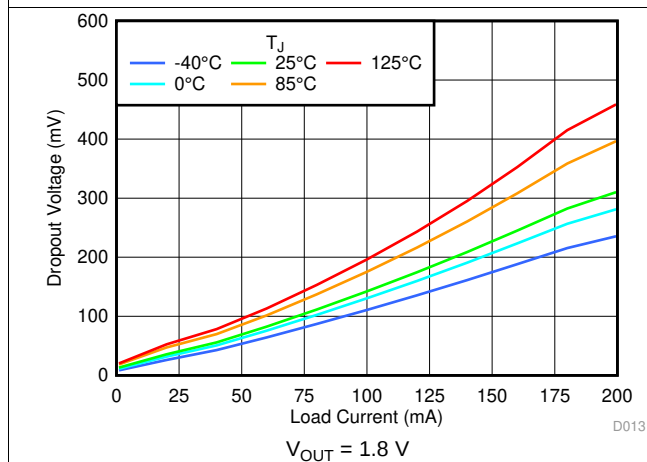
图 21. Dropout vs I_{OUT} and Temperature
