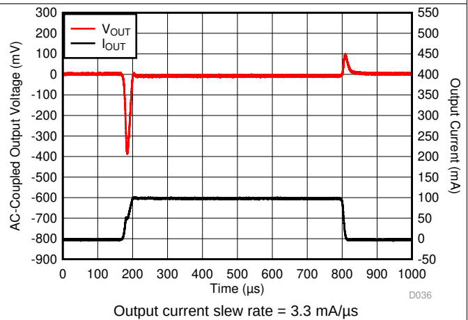
图 6. I_{OUT} Transient 0 mA to 100 mA
