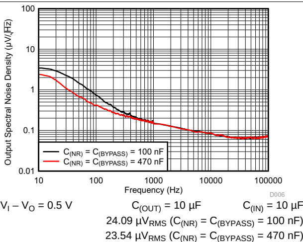
Figure 21. Output Spectral Noise Density vs Frequency (RMS noise (100 Hz to 100 kHz))
