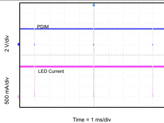
图 16. 99% Duty Cycle, 250 Hz PWM Dimming
