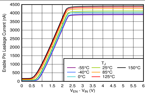
图 6-43. Enable Pin Leakage Current vs V_{EN} - V_{IN}
