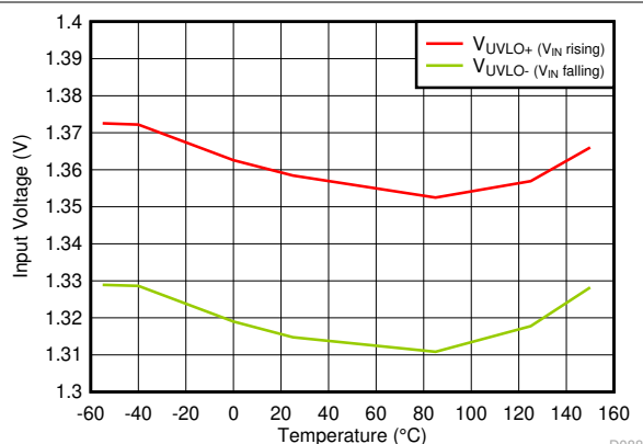
图 6-46. UVLO Threshold vs Temperature
