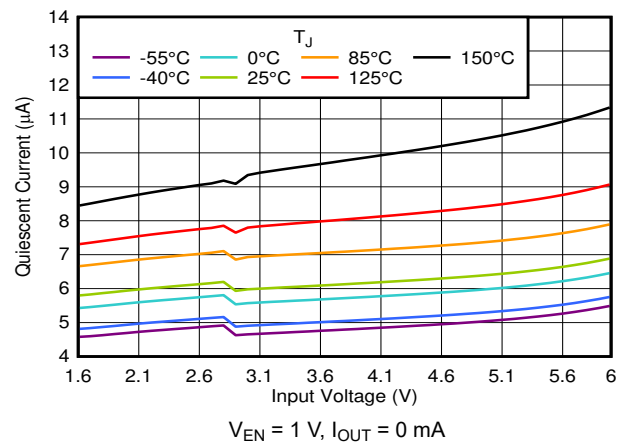
图 6-34. I_{GND} vs V_{IN}
