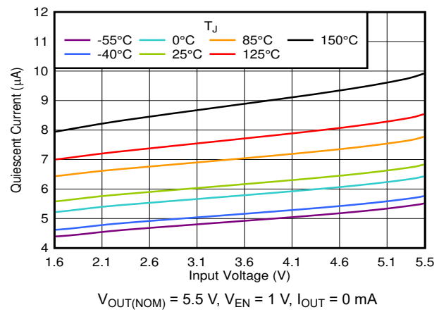
图 6-36. I_{GND} vs V_{IN} in the Dropout Region
