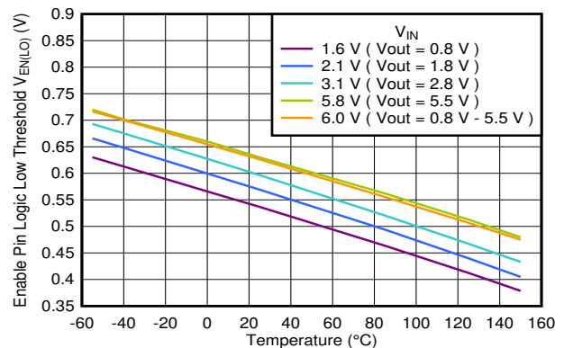
图 6-48. Enable Logic Low Threshold vs Temperature
