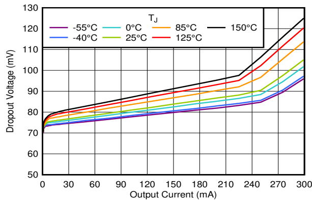
图 6-25. Dropout Voltage vs I_{OUT}
