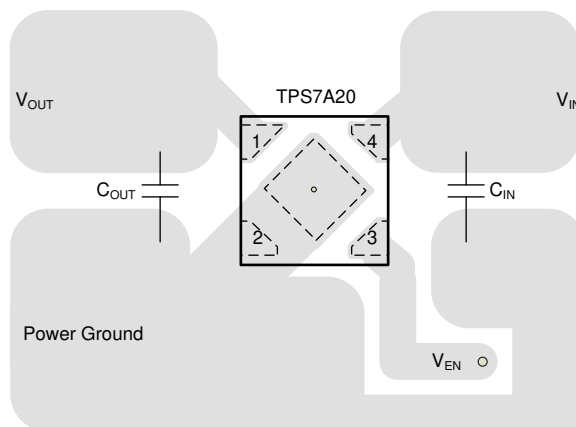
图 10-2. DQN Package (X2SON) Typical Layout
