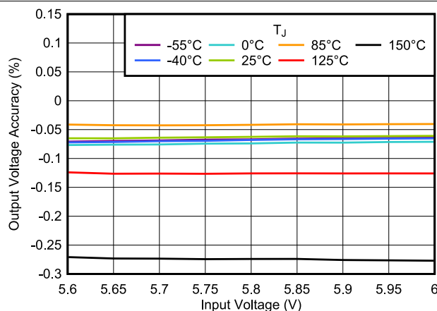
图 6-22. Output Voltage Accuracy vs V_{IN}
