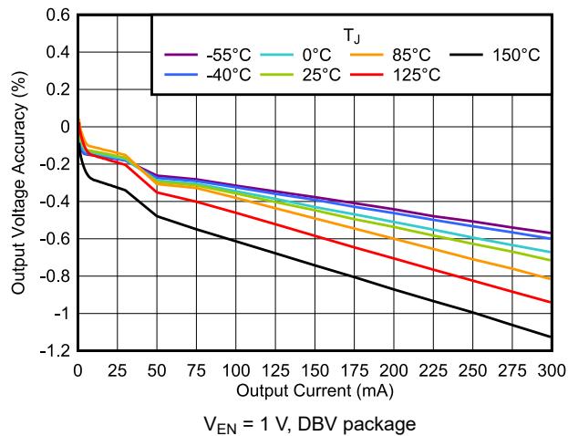
图 6-15. Output Voltage Accuracy vs I_{OUT}
