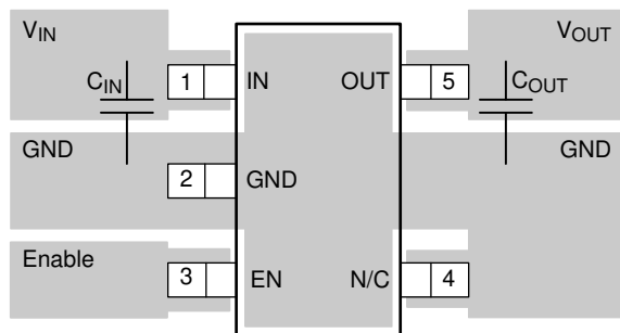
图 10-1. DBV Package (SOT-23) Typical Layout
