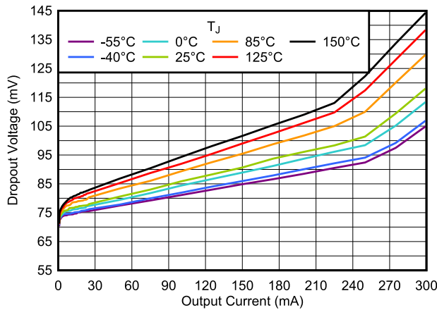
图 6-25. Dropout Voltage vs I_{OUT}
