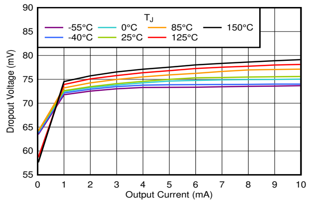
图 6-26. Dropout Voltage vs I_{OUT}
