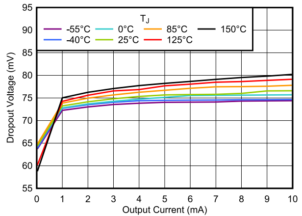
图 6-26. Dropout Voltage vs I_{OUT}
