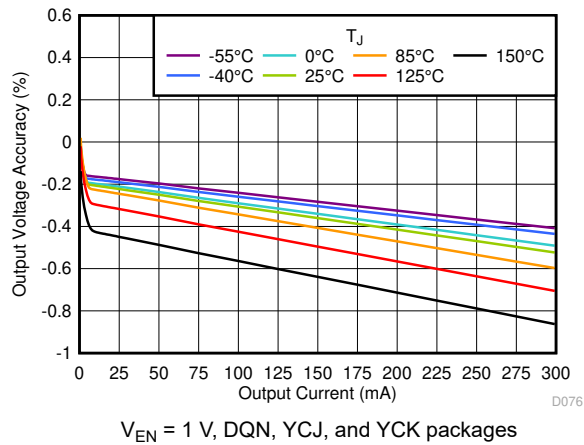
图 6-13. Output Voltage Accuracy vs I_{OUT}
