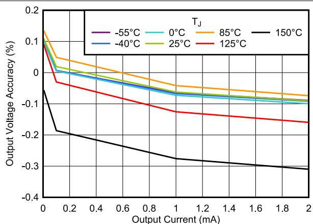
图 6-20. Output Voltage Accuracy vs I_{OUT}
