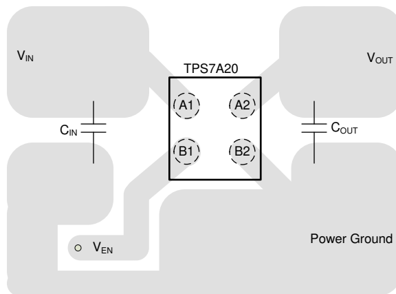
图 10-3. YCJ and YCK Package (DSBGA) Typical Layout
