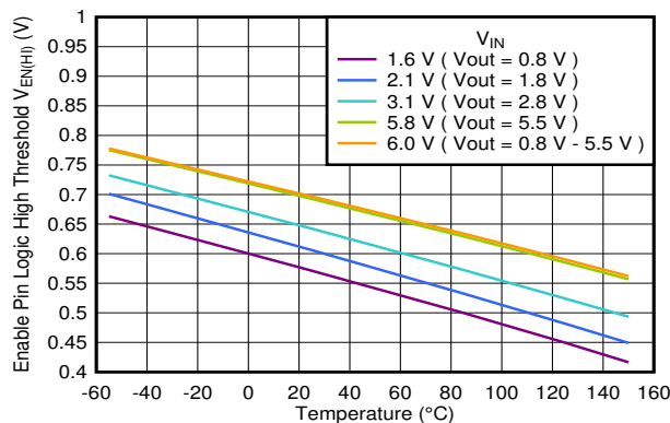
图 6-47. Enable Logic High Threshold vs Temperature
