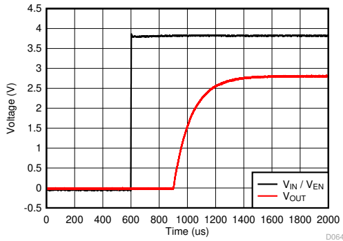
图 8-5. Start-Up
