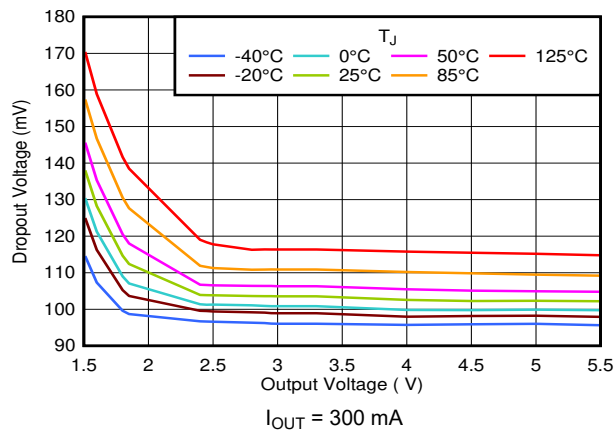
图 6-33. Dropout Voltage vs V_{OUT}
