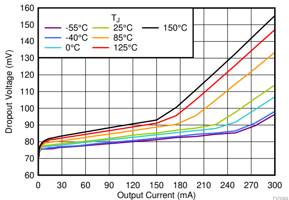
图 6-27. Dropout Voltage vs I_{OUT}
