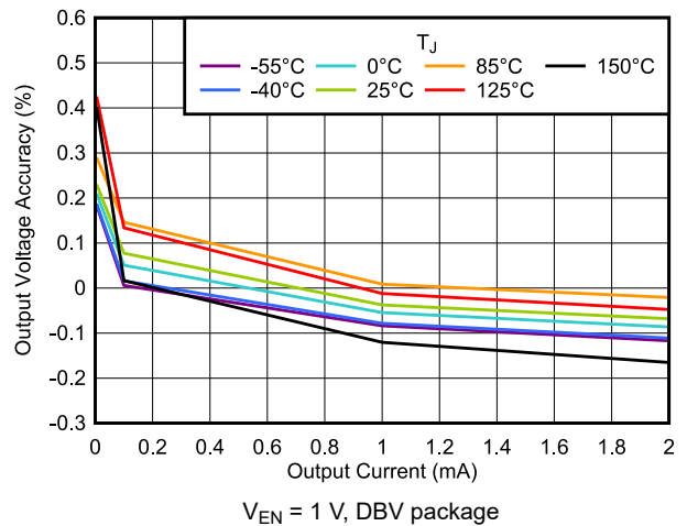
图 6-16. Output Voltage Accuracy vs I_{OUT}
