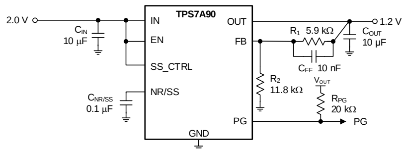
图 39. Application Example
