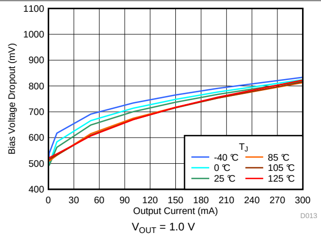
图 8. Dropout vs V_{BIAS} and Temperature
