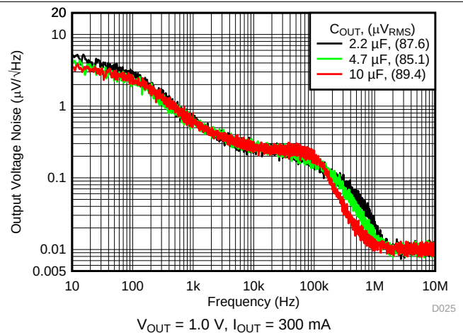
图 34. Output Noise vs Frequency and C_{OUT}
