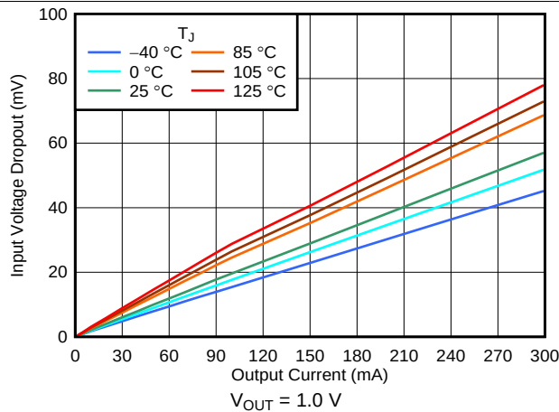
图 7. Dropout vs I_{OUT} and Temperature, DSE Package
