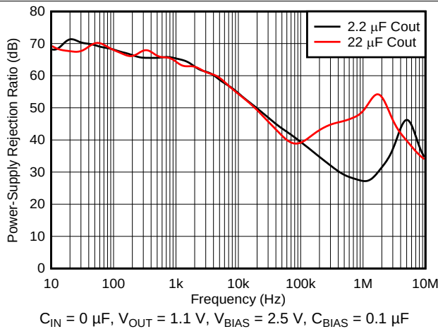
图 27. PSRR vs Frequency and C_{OUT}
