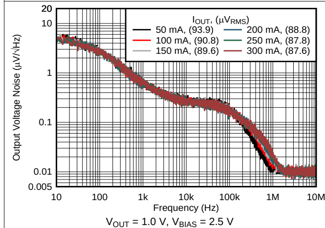
图 33. Output Noise vs Frequency and I_{OUT}
