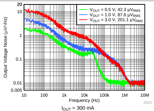
图 32. Output Noise vs Frequency and V_{OUT}
