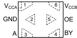
图 5-5. DTQ Package 6-Pin X2SON Transparent Top View
