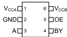
图 5-3. DRL Package 6-Pin SOT-5X3 Transparent Top View
