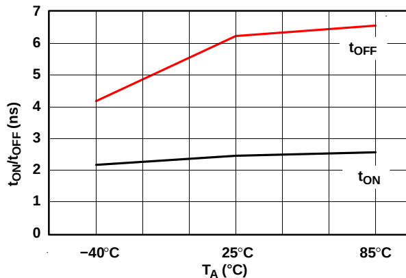
Figure 8. t ON and t OFF vs Temperature (V + = 5 V)
