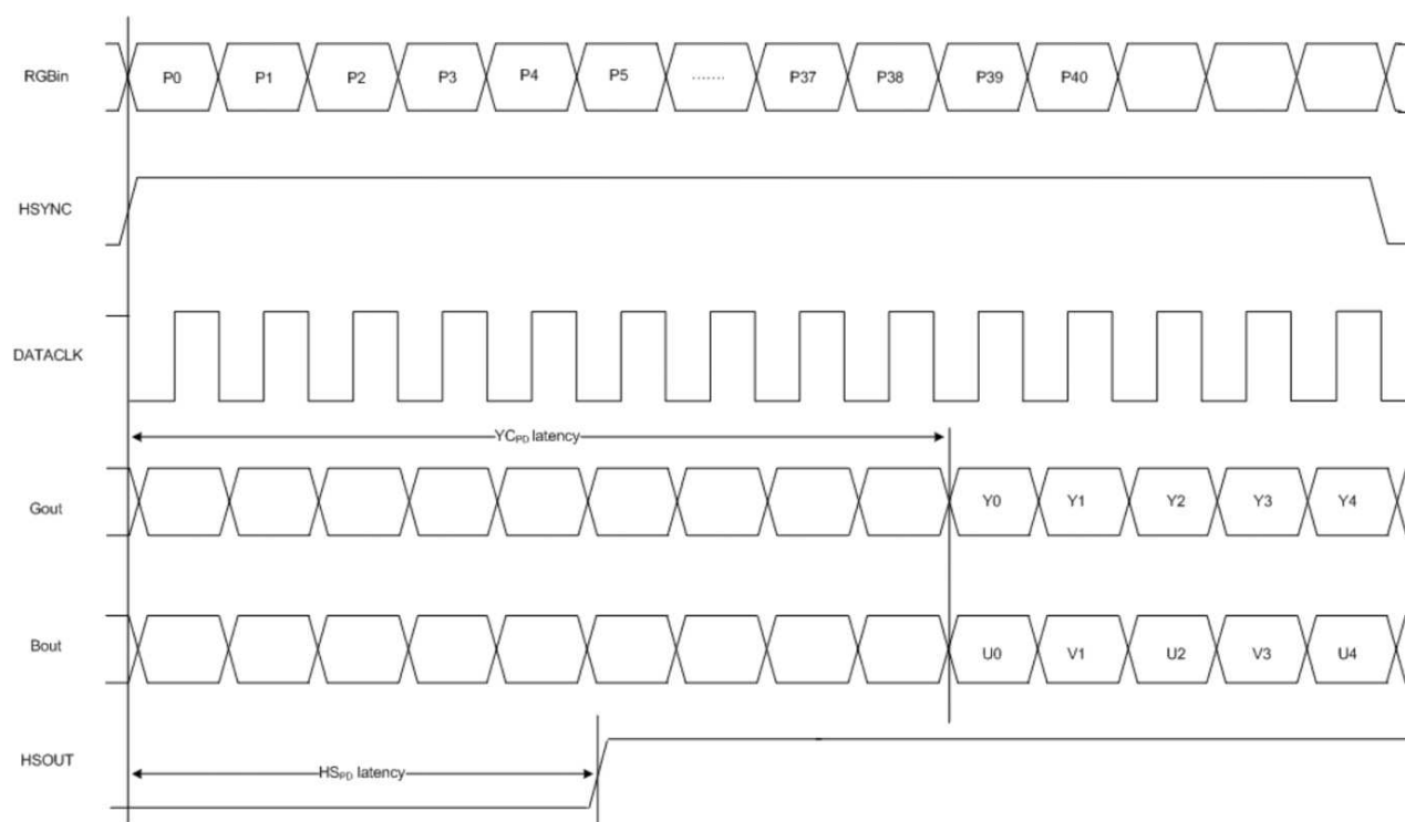
Figure 6. Output Timing Diagram
