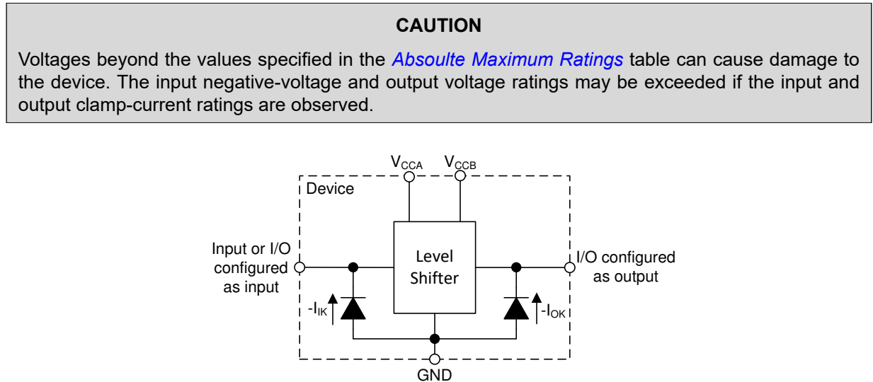
图 9-2. Electrical Placement of Clamping Diodes for Each Input and Output
