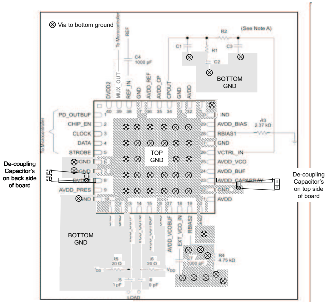
Figure 91. TRF3761 Layout
