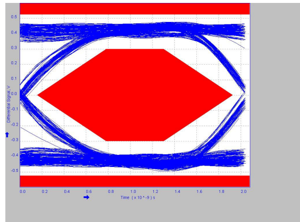
Figure 8-19. 2 Meter Post-Channel With TUSB216 BOOST=1 RX_SEN=HIGH
