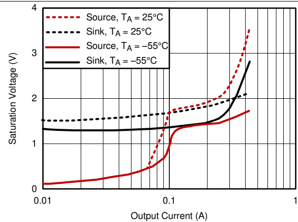
Figure 8. Output Saturation
