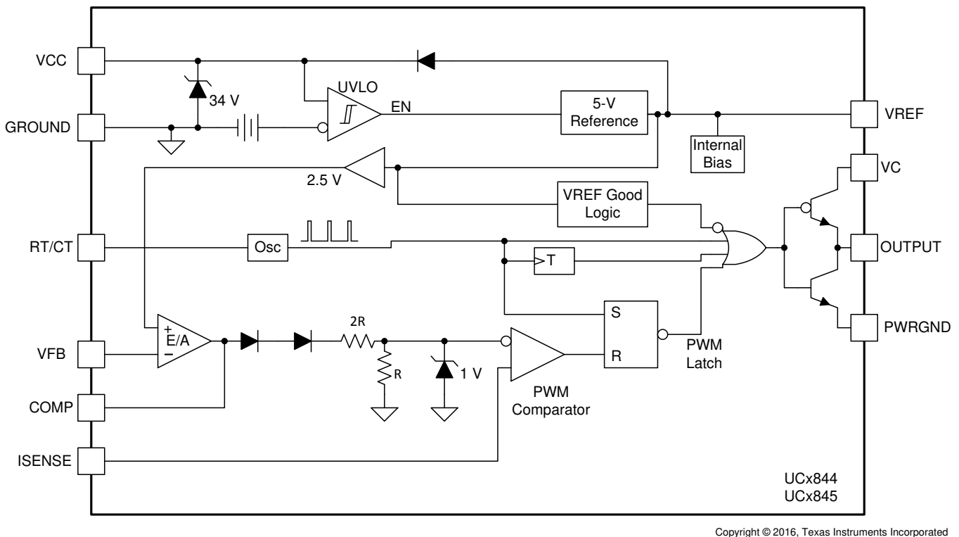
Figure 12. UCx844 and UCx845 Block Diagram, Toggle
