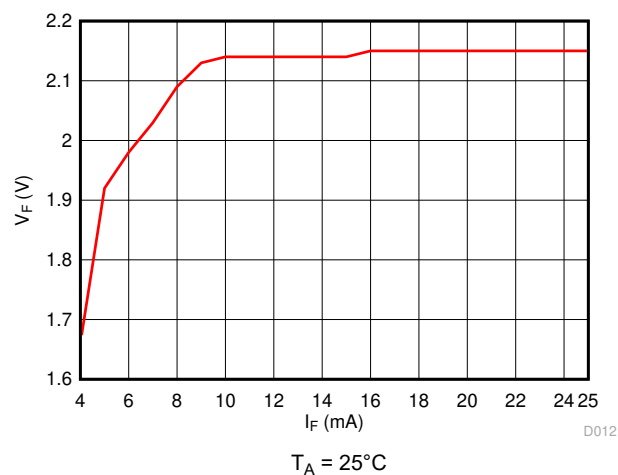
图 6-15. Forward current versus Forward voltage drop
