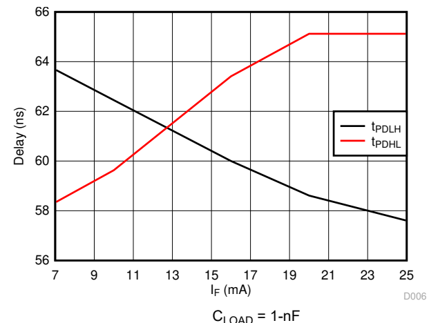
图 6-9. Propagation delay versus Forward current
