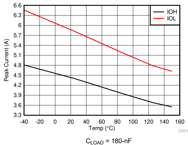
图 6-4. Output Drive currents versus Temperature
