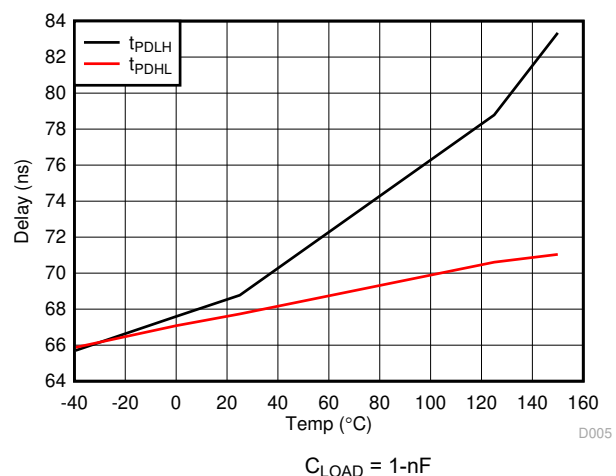
图 6-8. Propagation delay versus Temperature
