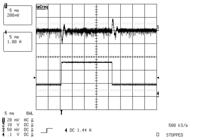
CH1: Output Voltage AC Coupled, 200 mV/div CH4: Output Current, 1 A/div Figure 38. Output Voltage During 0.9-A to 2.7-A Load Transient
