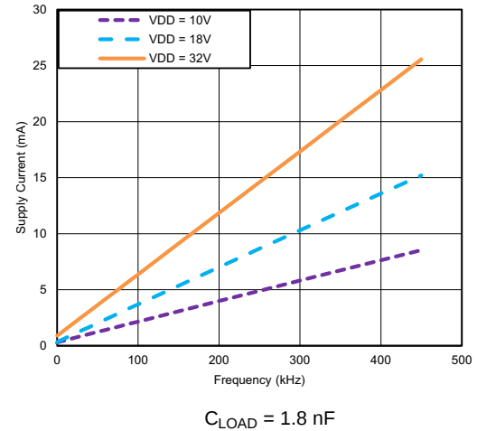
图 9. Operating Supply Current vs. Frequency
