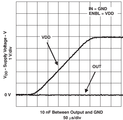
Figure 25. Output Behavior vs V_{DD} (Noninverting)
