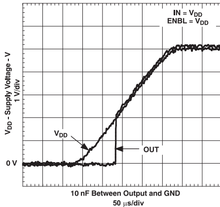
Figure 23. Output Behavior vs V_{DD} (Noninverting)
