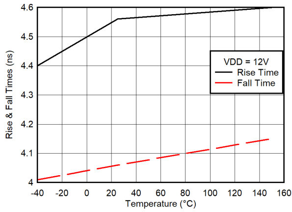
图 6-8. Output Rise and Fall Time vs Temperature
