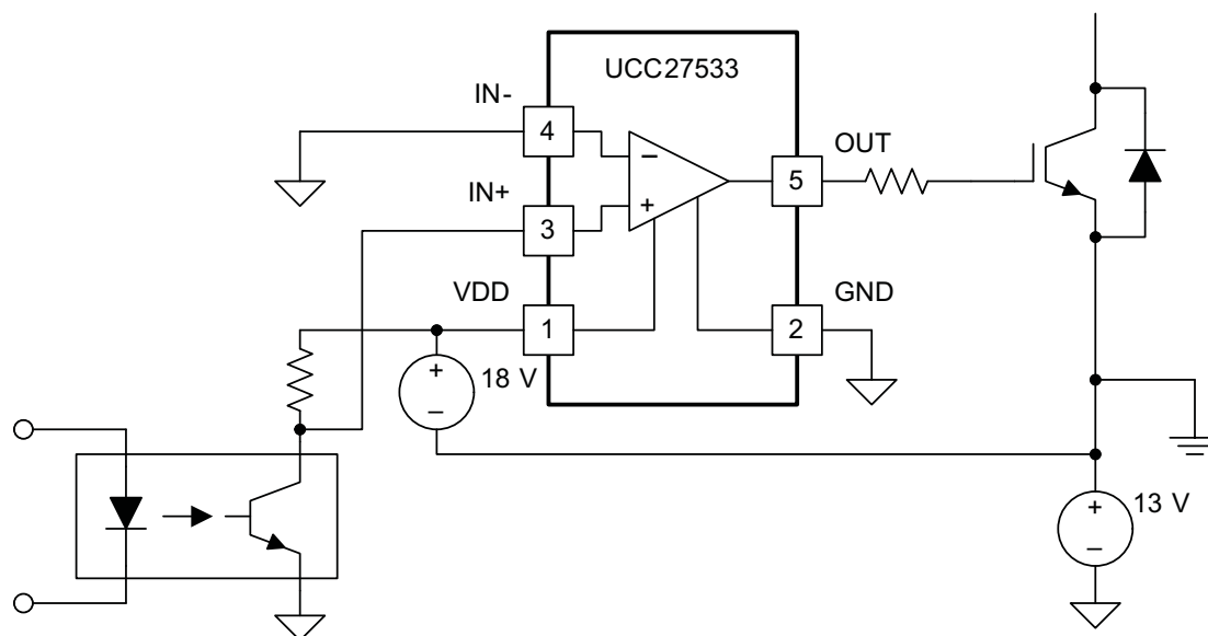
图 46. Single-Output Driver
