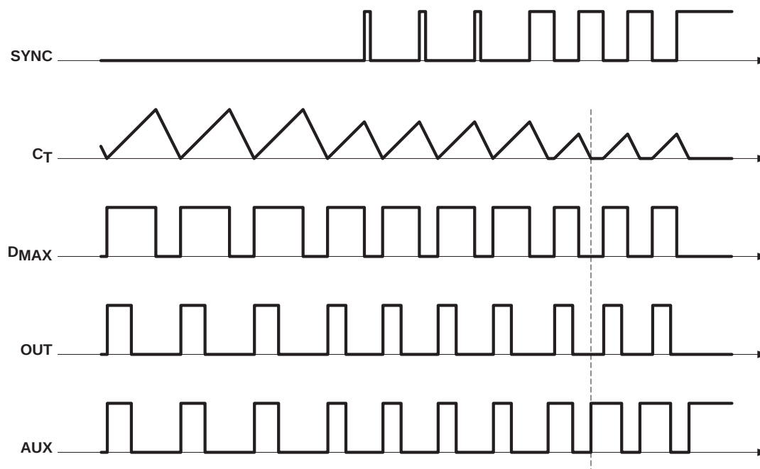
Figure 6. Synchronization Waveforms, P-Channel
