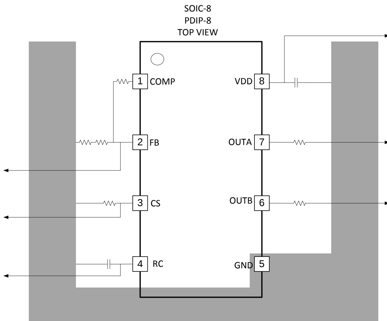
Figure 9. Layout Example
