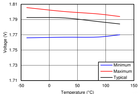
图 8-8. BP18 Voltage vs Temperature
