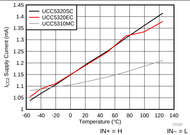
图 18. I_{CC2} Supply Current vs Temperature
