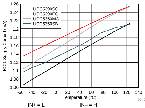
图 11. I_{CC1} Supply Current vs Temperature
