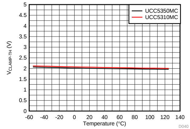
图 24. UCC5310M V_{Clamp} vs Temperature
