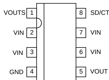
DP PACKAGE (FRONT VIEW)
