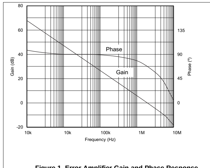
Figure 1. Error Amplifier Gain and Phase Response
