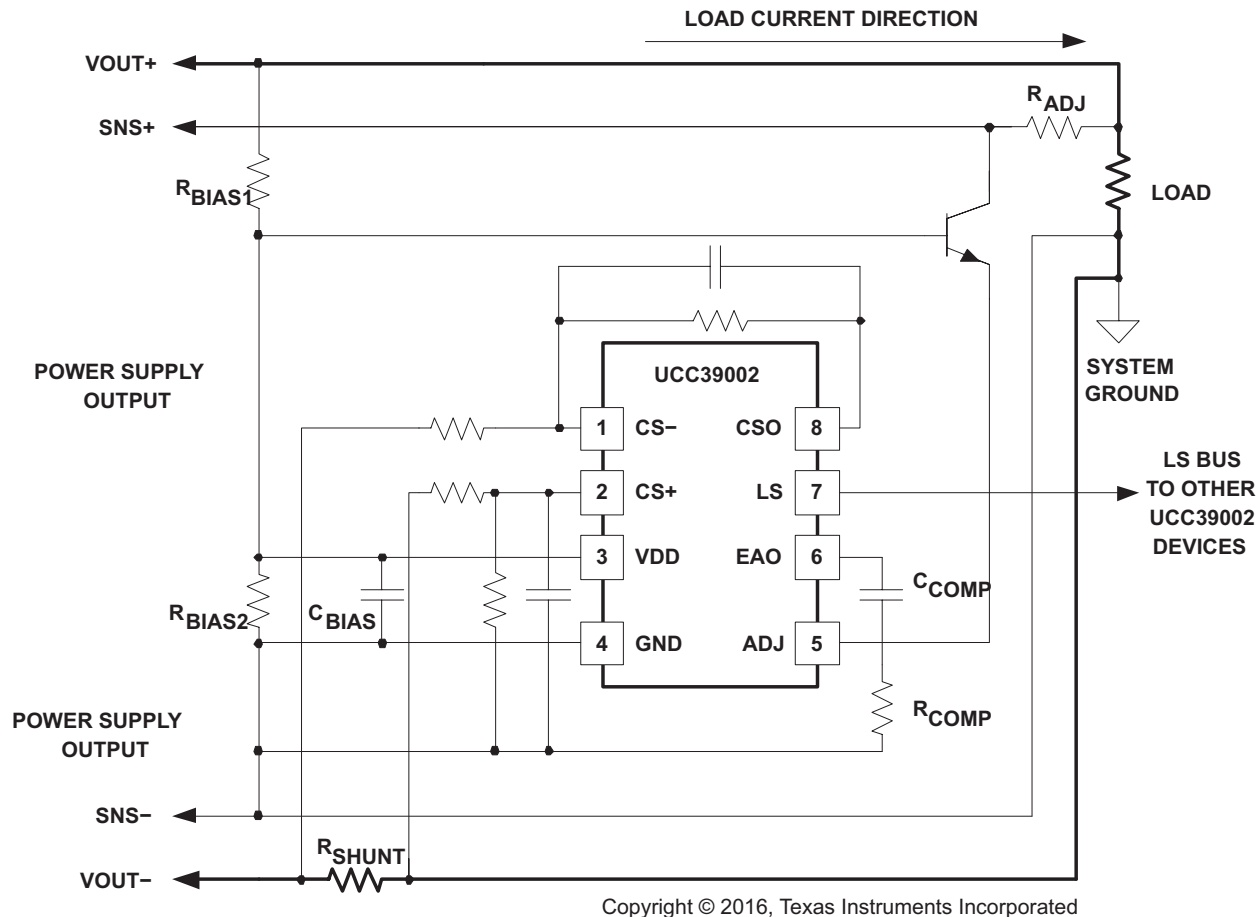
Figure 5. High Voltage Application
