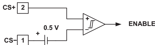
Figure 2. Enable Comparator
