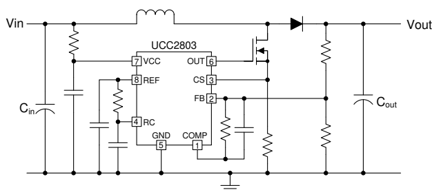
Simplified Application Diagram
