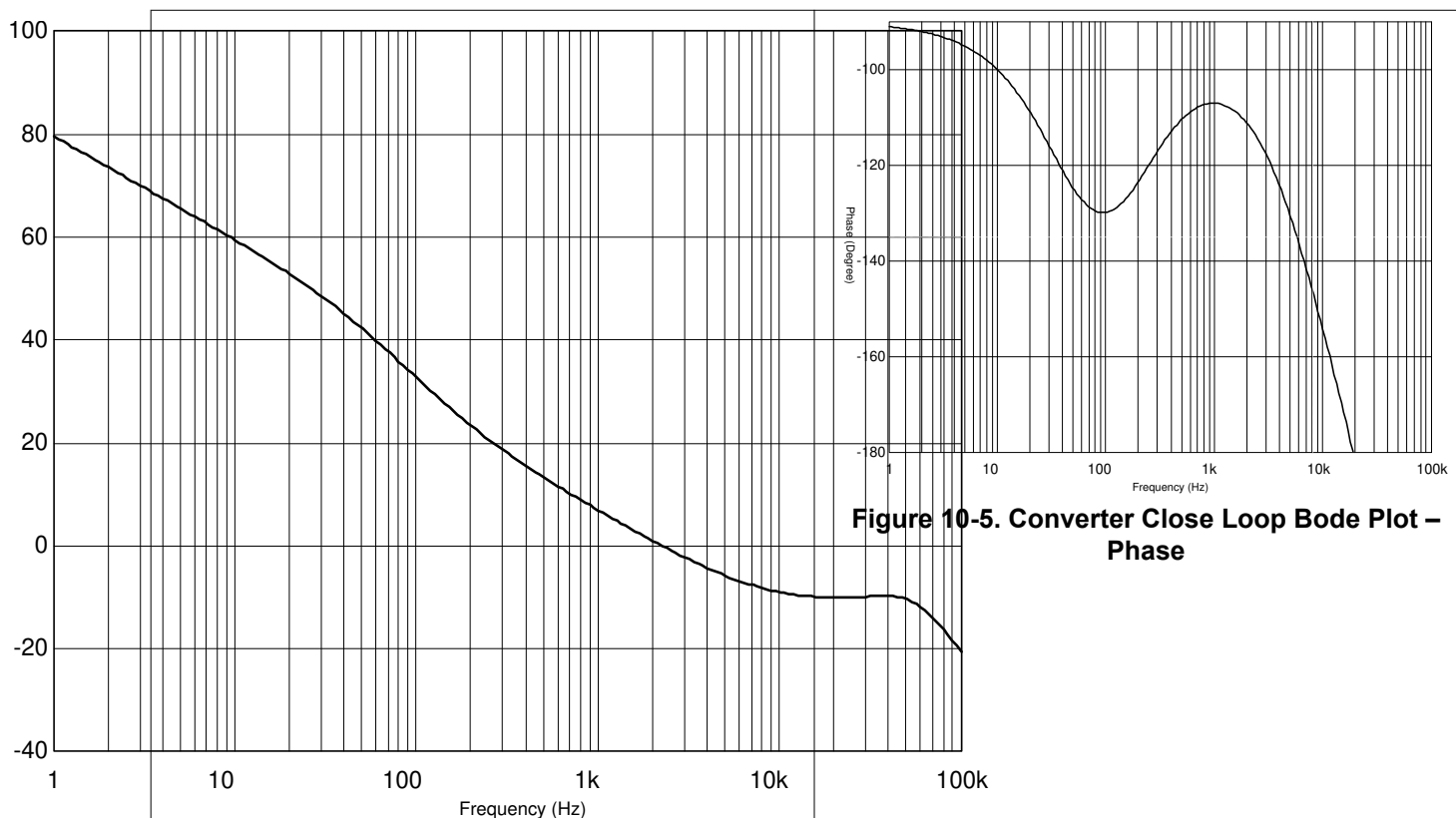
Figure 10-4. Converter Close Loop Bode Plot – Gain
