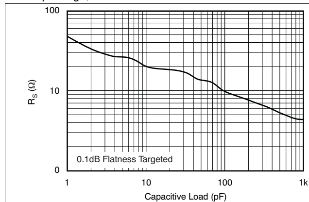
Figure 29. Recommended R_S vs Capacitive Load
