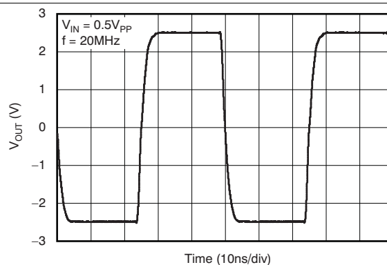
Figure 34. Large-Signal Pulse Response
