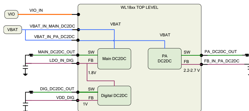
Figure 5-1. Internal DC2DCs
