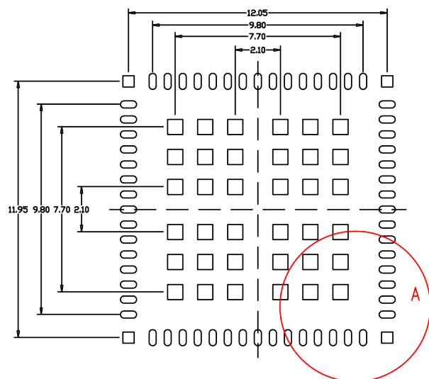
Figure 4-2. Outline of 100-Pin MOC Package
