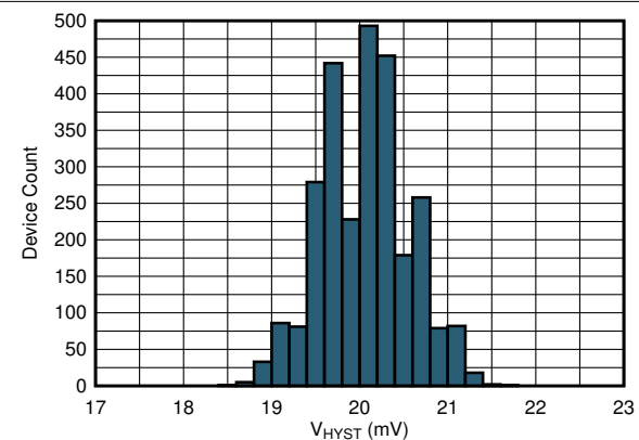
TLV40x1R2 V_S = 5\text{ V} 图 7-12. Hysteresis Histogram
