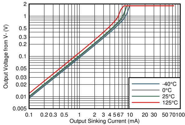
V_S = 1.8\text{V} 图 7-21. Output Voltage vs Output Sinking Current
