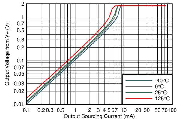
V_S = 1.8\text{V} 图 7-22. Output Voltage vs Output Sourcing Current
