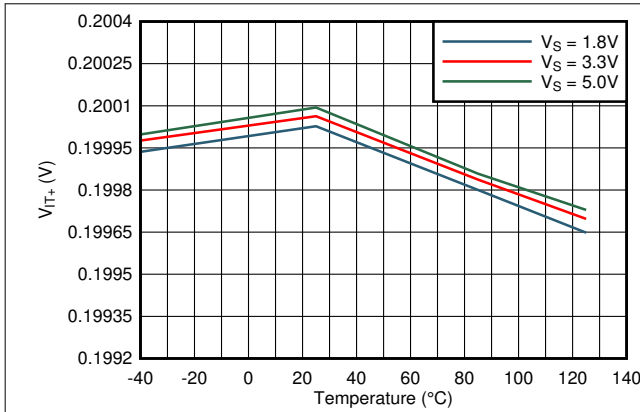
TLV40x1R2 图 7-7. Positive Threshold vs Temperature
