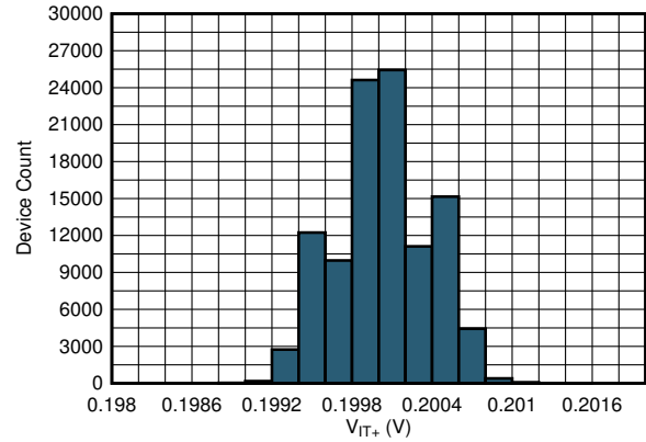
TLV40x1R2 V_S = 5\text{ V} 图 7-8. Positive Threshold Histogram
