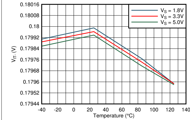
TLV40x1R2 图 7-9. Negative Threshold vs Temperature
