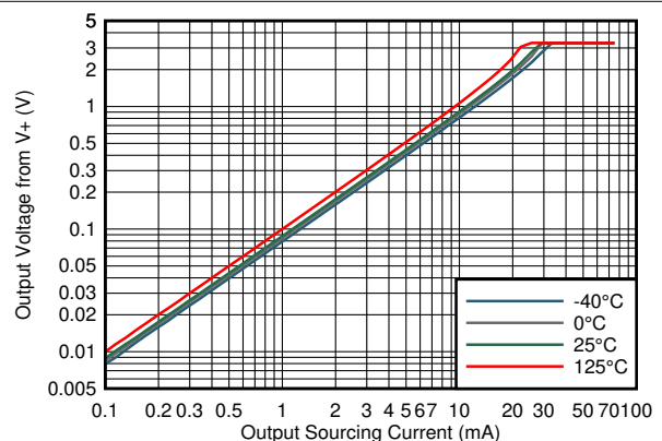
V_S = 3.3\text{V} 图 7-24. Output Voltage vs Output Sourcing Current
