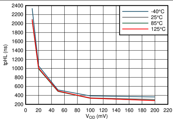
图 7-29. Propagation Delay High-Low vs Input Overdrive
