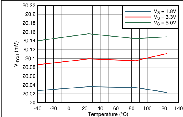
TLV40x1R2 图 7-11. Hysteresis vs Temperature
