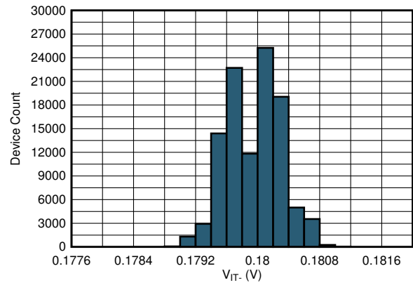
TLV40x1R2 V_S = 5\text{ V} 图 7-10. Negative Threshold Histogram
