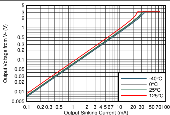
V_S = 3.3\text{V} 图 7-23. Output Voltage vs Output Sinking Current
