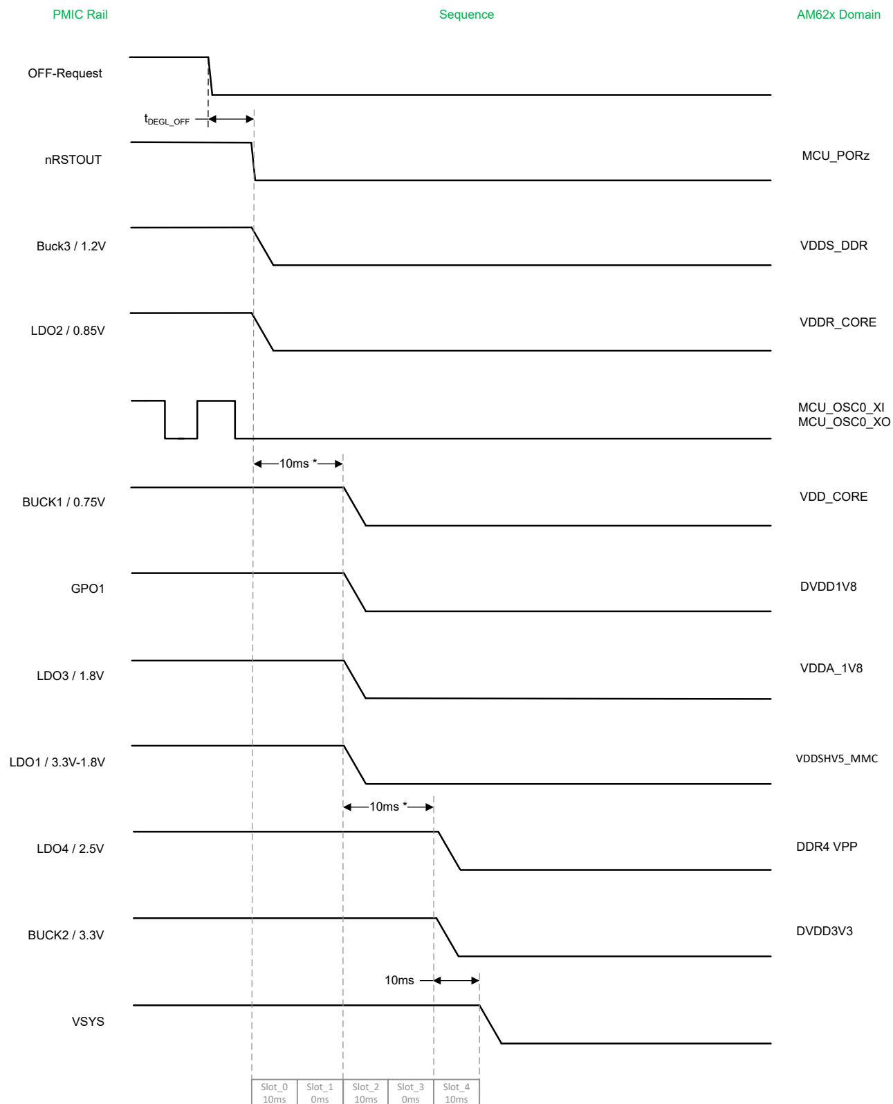
图 7-3. Power-down sequencing (example)
