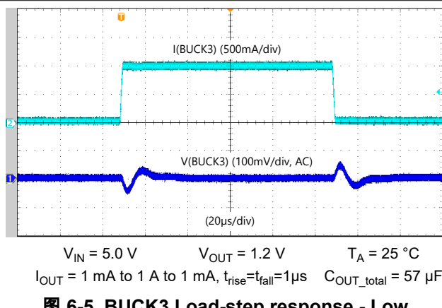
图 6-5. BUCK3 Load-step response - Low Bandwidth, forced PWM
