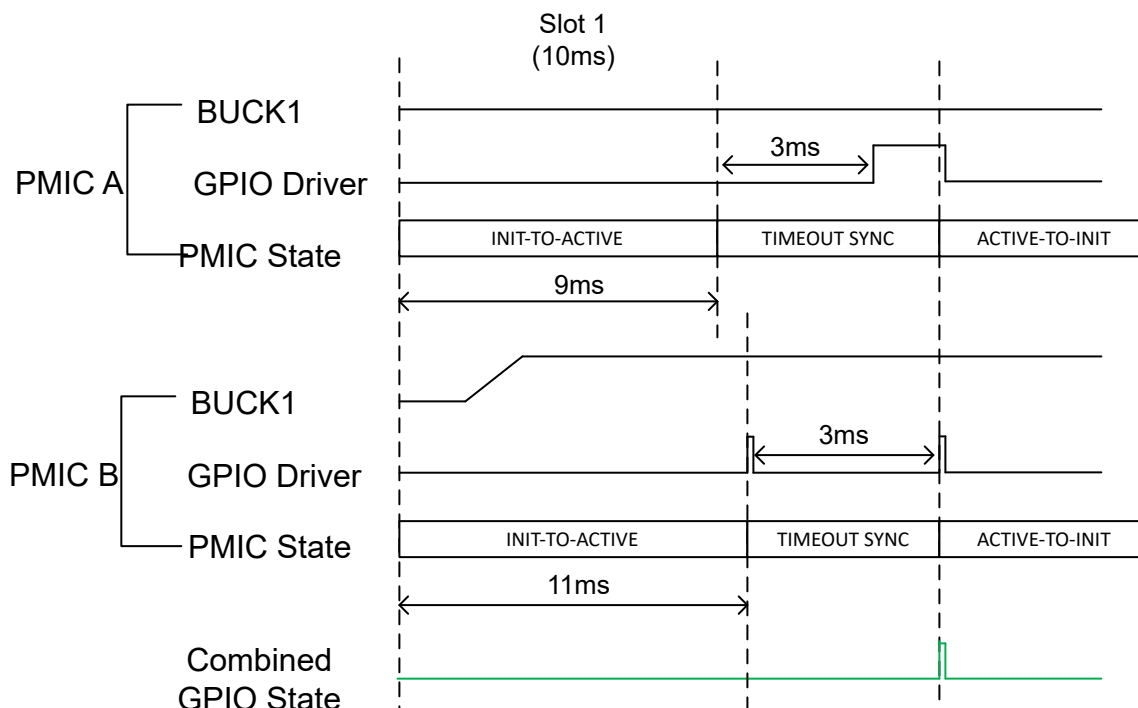
Figure 8-7. Timeout Synchronization
