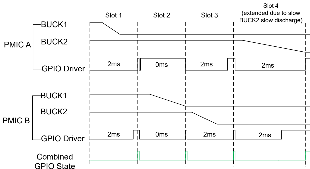
图 8-6. Synchronization during power-down sequence
