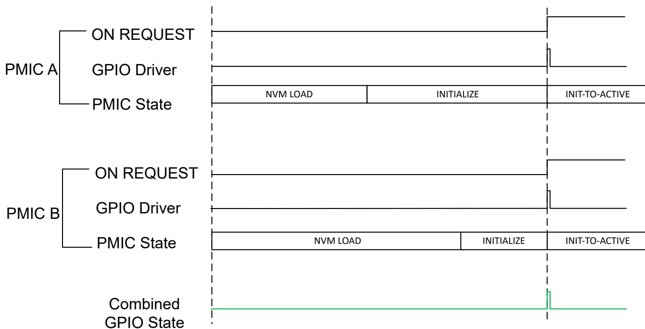
图 8-3. Synchronization before Power-up
