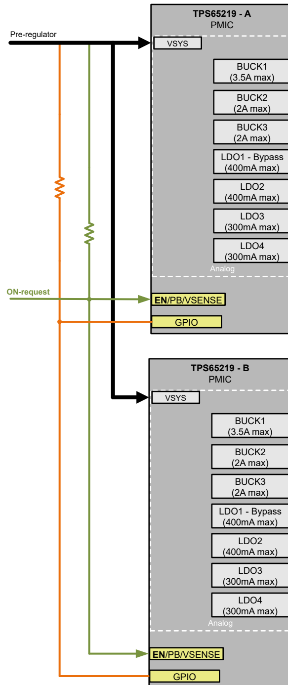
图 8-2. Multi-PMIC Configuration Example
