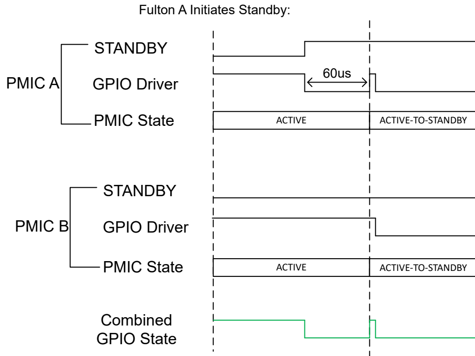
图 8-5. Synchronization before transitioning to Standby/OFF request/COLD RESET
