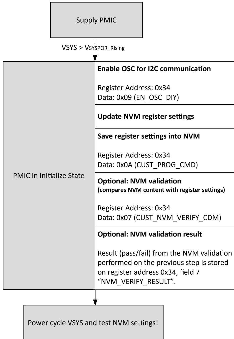
图 8-8. NVM Programming steps
